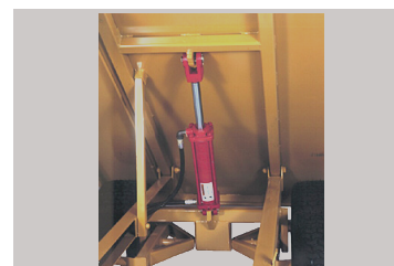
Cylinder and safety lock bracket
